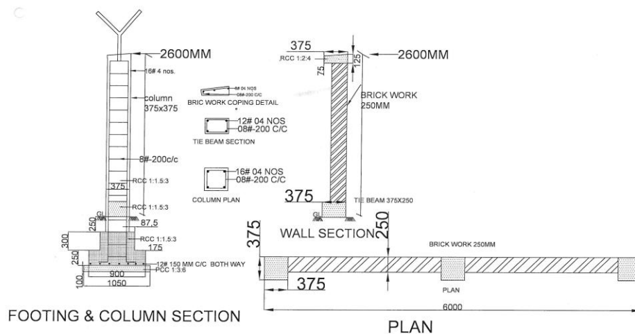
DETAILS OF NEW BOUNDARY WALL
