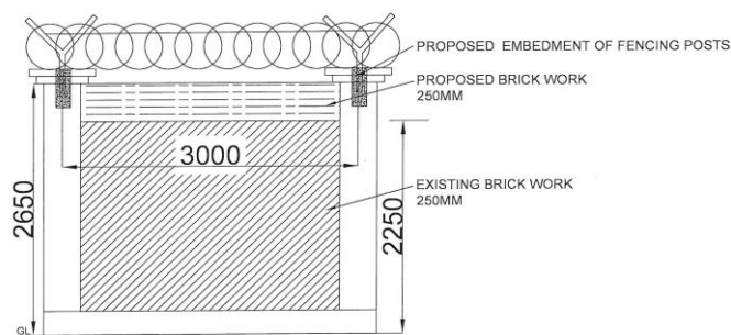
TYPICAL DETAILS MODIFICATION FOR EXISTING BOUNDARY WALL FOR A SINGLE SPAN
