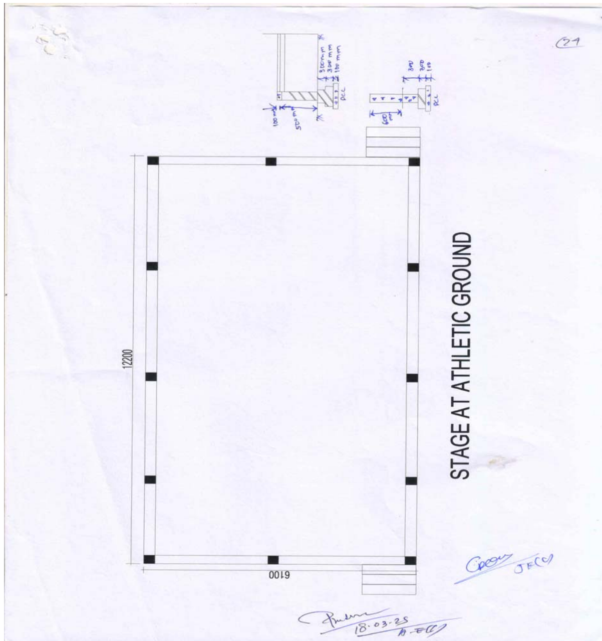
Drawing for construction of stage
