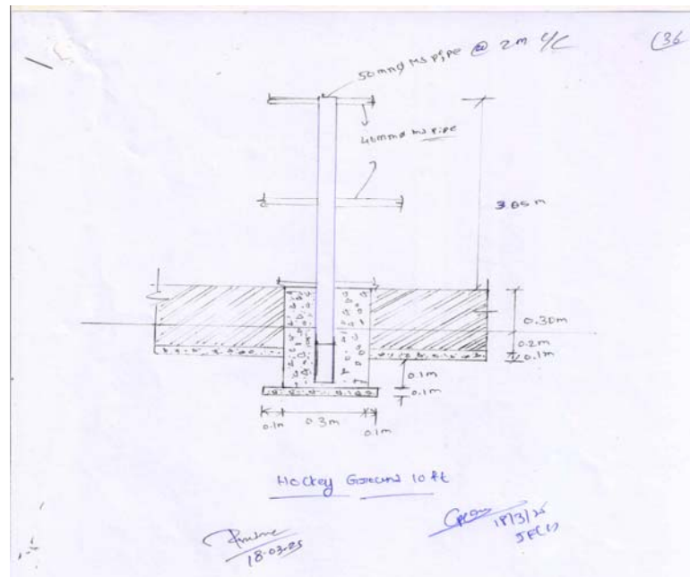
Cross Section of fabric fencing of Hockey ground
