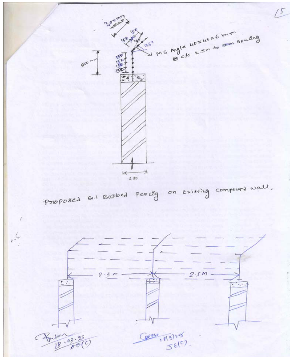
Schematic drawing for barbed wire fencing around Swimming Pool
