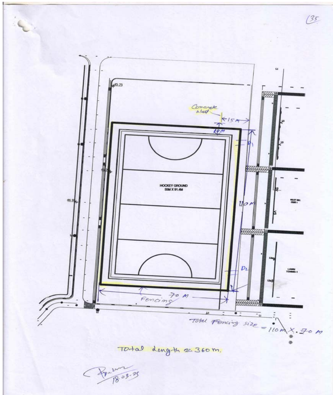
Layout drawing of fabric fencing of Hockey ground
