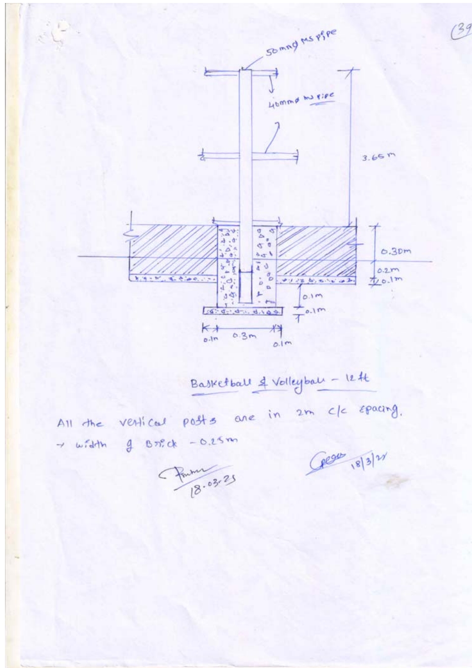
Cross section of fabric fencing of basketball and volleyball court
