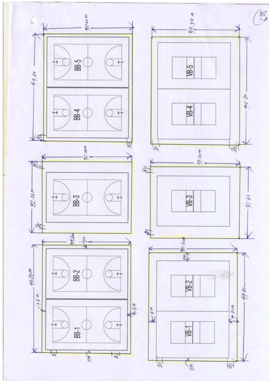
Layout drawing of fabric fencing of Basketball and Volley Ball court
