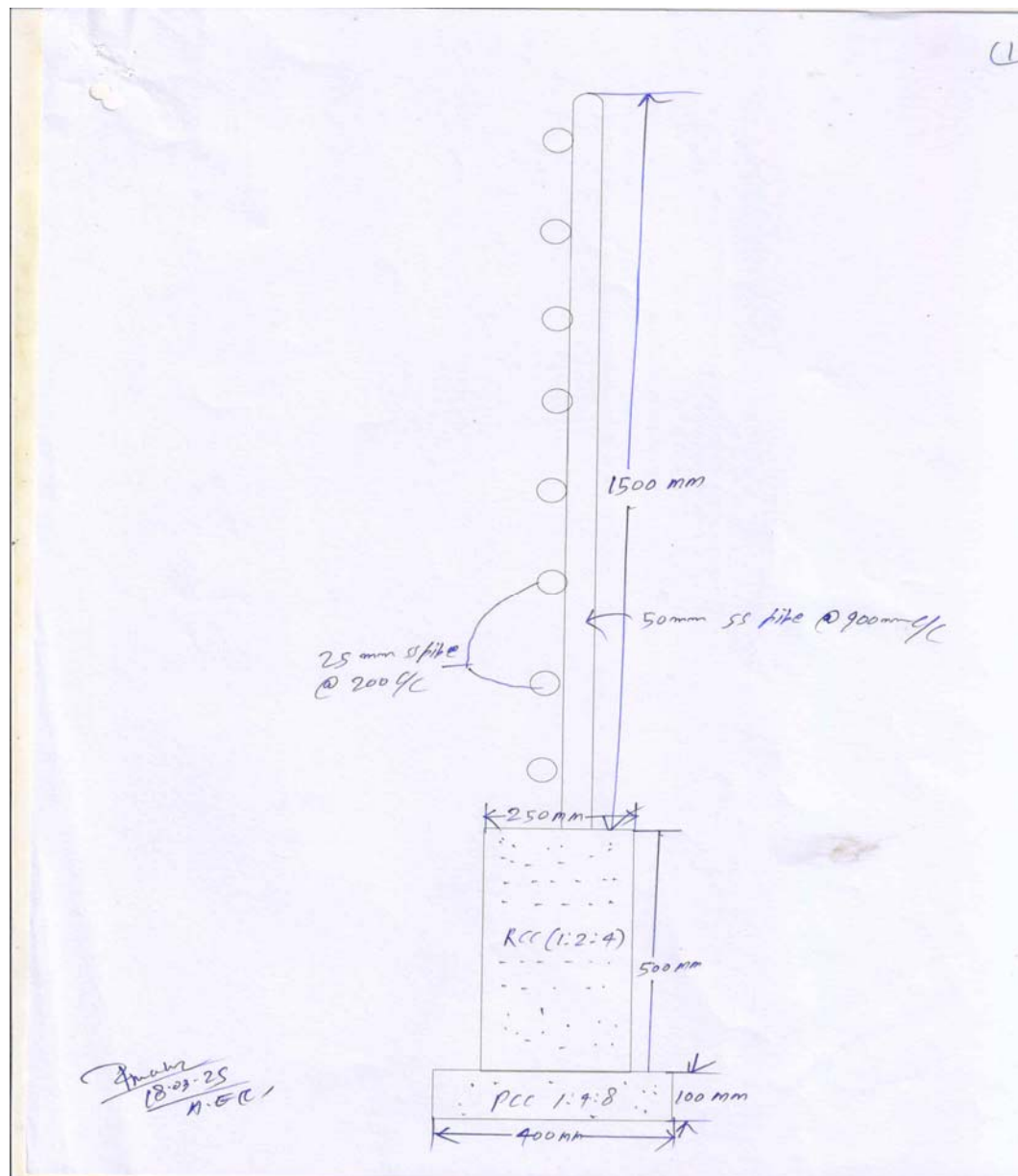
Cross section of Railing of Swimming Pool
