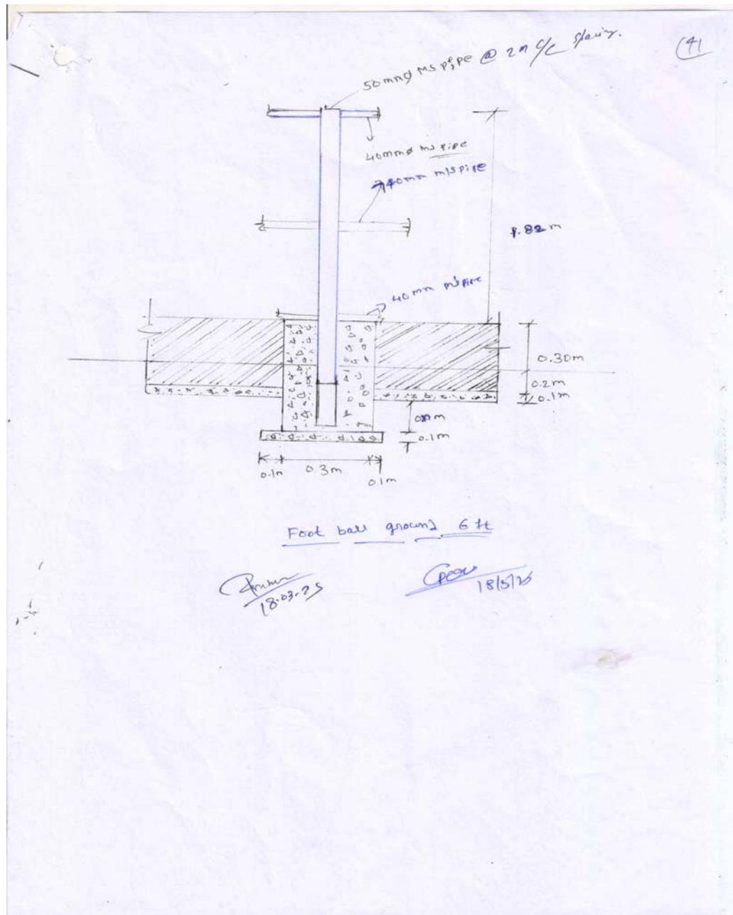
Schematic drawing of cross section of chain link fabric fencing
