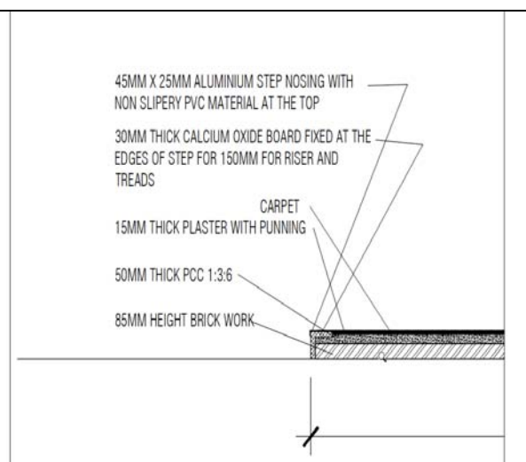
Typical details of Step-1 at SMS/SEOCS/SMME
