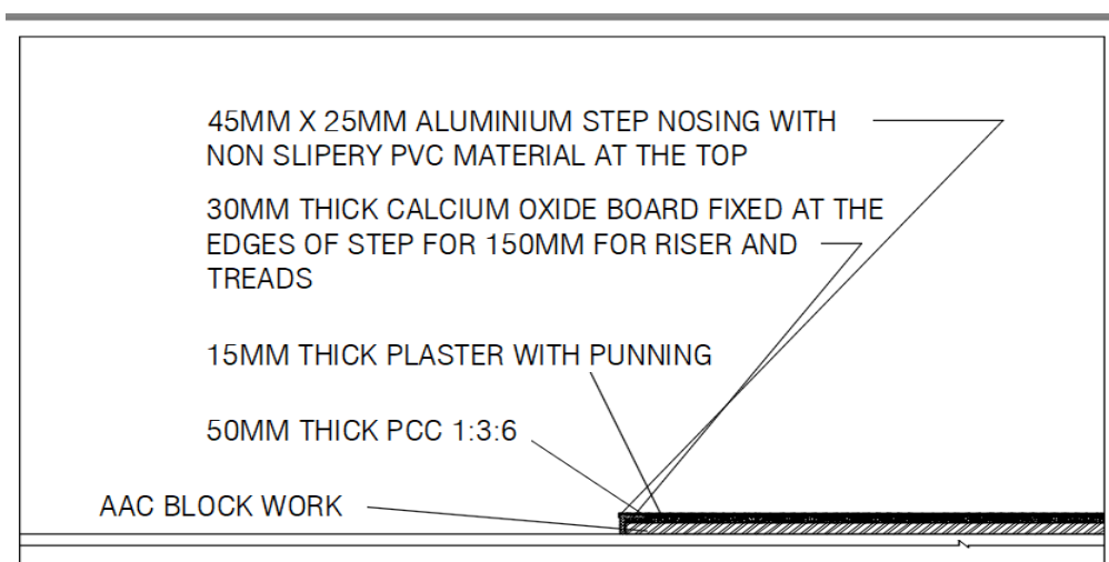
TYPICAL STEP DETAILS OF SEMINAR ROOM AT SIF
