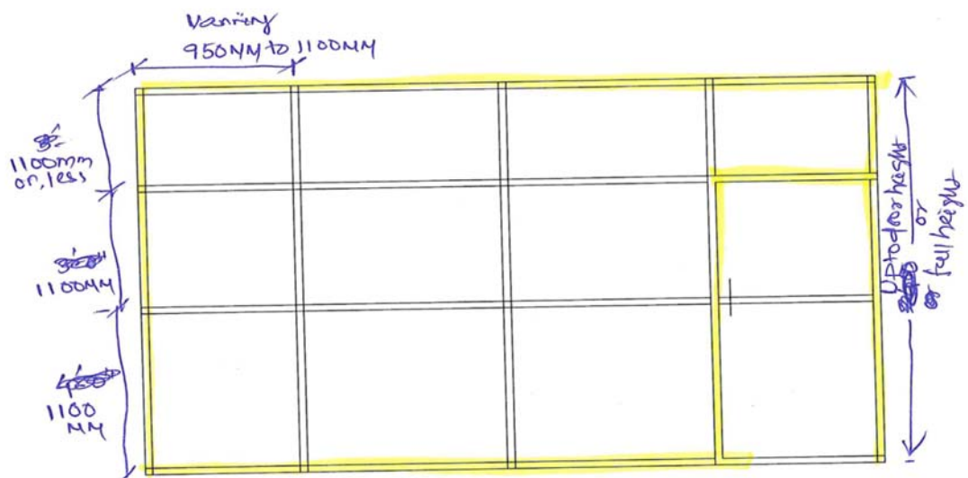
TYPICAL DETAIL OF PARTITION UP TO 8 FEET / Full height
