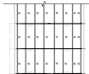
STEEL ROOF LEVEL PLAN TYPICAL PART PLAN CYCLE PARKING G1 80 (M) PIPE (NOT SHOWN IN PLAN, REF. SEC F1-F1) G11 80 (M) PIPE P1 33 WIDE x 66 DEEP x 2.9mm THK
